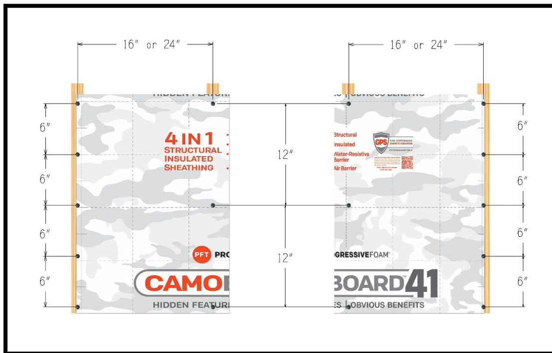
CAMOBOARD FASTENING INSTALLATION DETAIL
